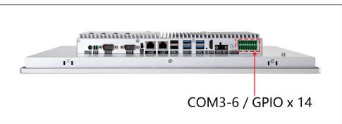
Optional I/O View : iDOOR-4x COM / 14xGPIO
